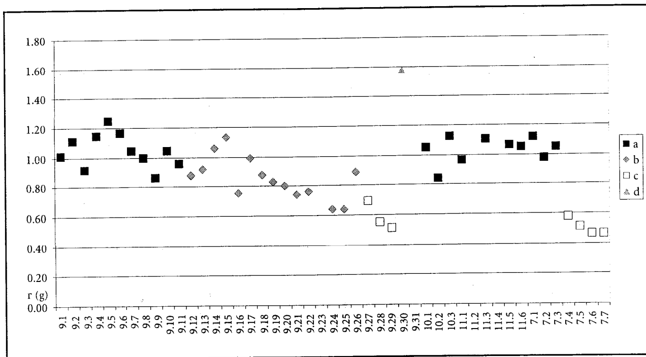
Chart 5: Average weights of coins from the time of the Emperor Uroš:
