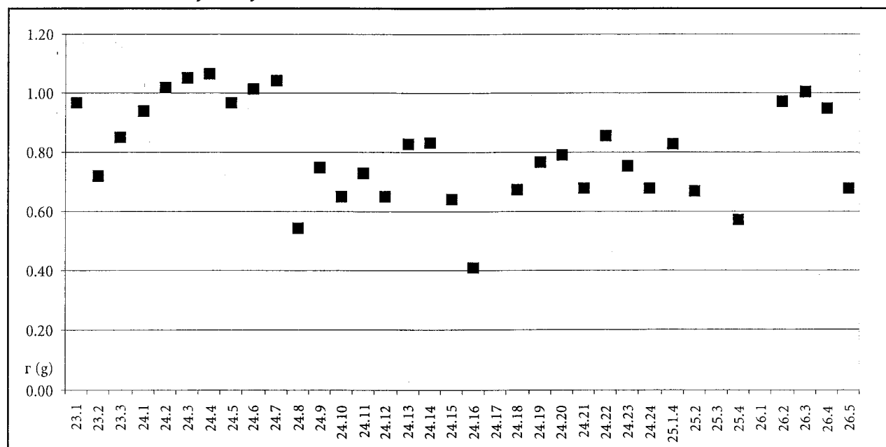
Chart 7: Average weights of dinars of Župan Nikola Altomanović, Prince Lazar and Djurdj I Balšić
