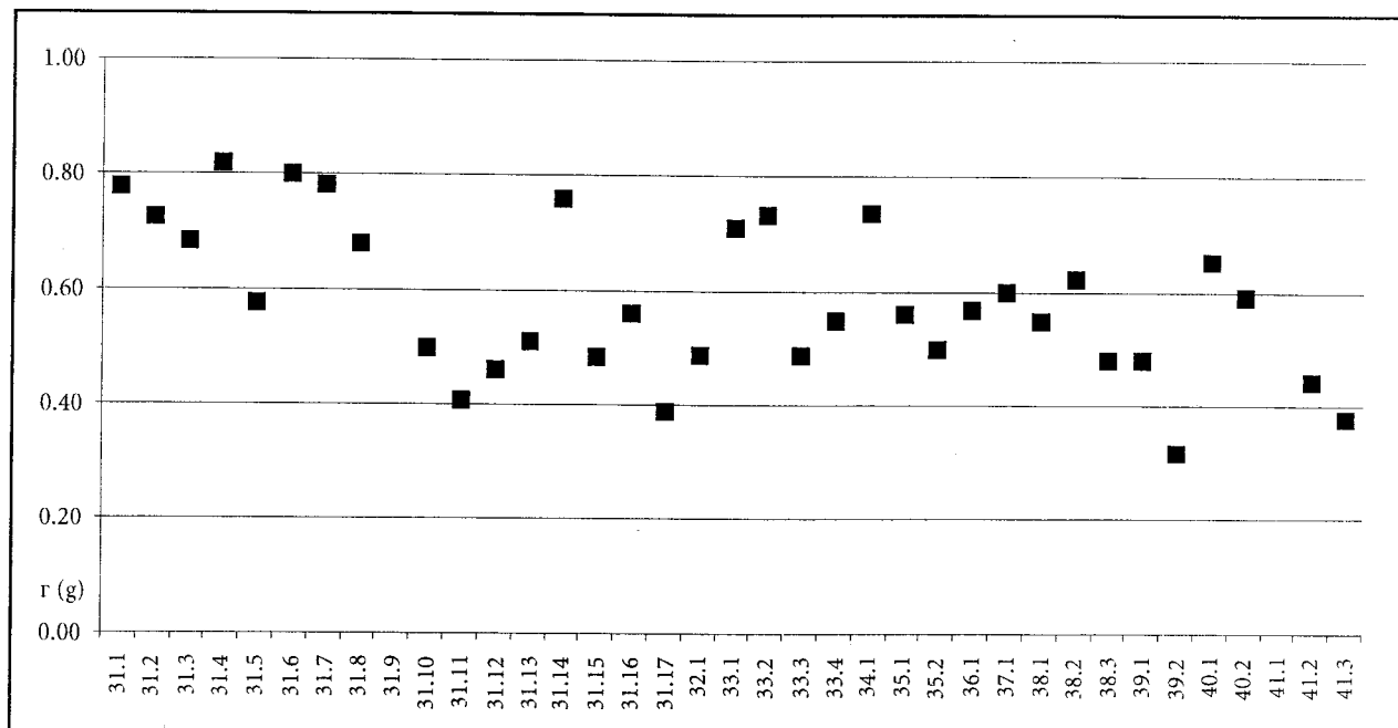
Chart 8: Average weights of dinars of Vuk Branković, local feudal lords, Patriarch and towns
