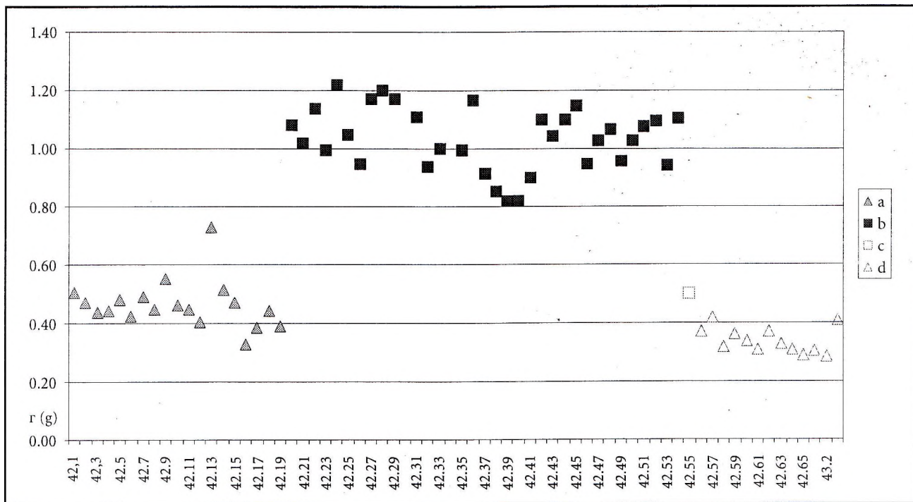
Chart 9: Average weights of coins of Stefan Lazarević:
