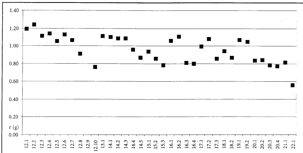
Chart 6: Average weights of dinars of King Vukašin and local rulers of southern Serbian lands
