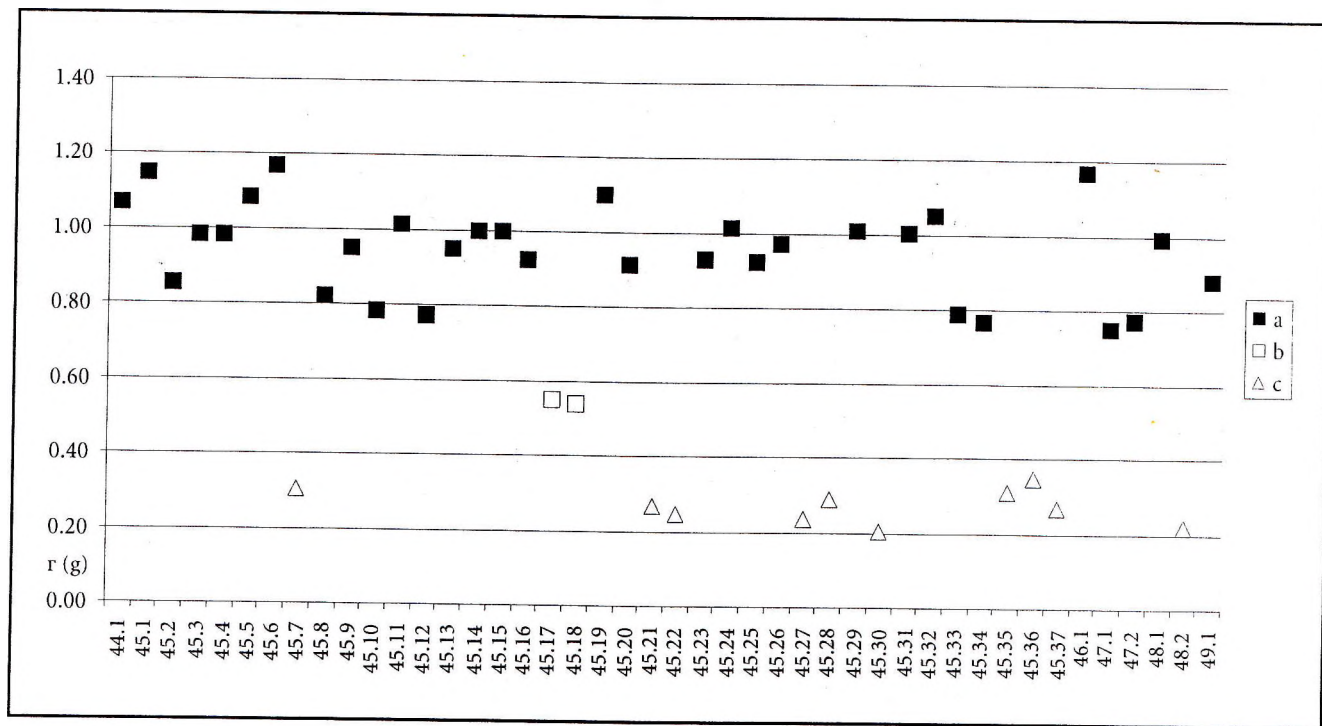
Chart 10: Average weights of coins of Djurdj Branković and Lazar Branković:
